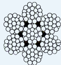
Cross Section 7 strands, 19 wires per strand = 133 wires
